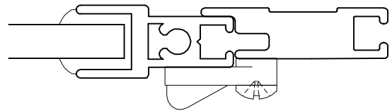
2 JAMB DETAIL SCALE: FULL
